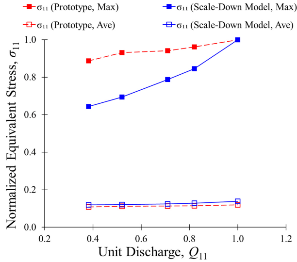
Fig. 14. Comparison of normalized equivalent stress in the scale-down and prototype runners according to discharge conditions
