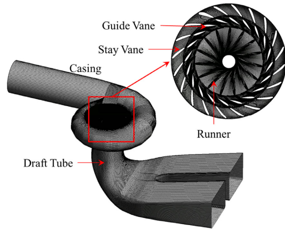
Fig. 6. Numerical grids for Francis hydro turbine components for the CFD analysis
