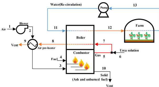
Fig. 1. Schematic diagram of a livestock manure solid fuel combustion boiler system for farm heating
