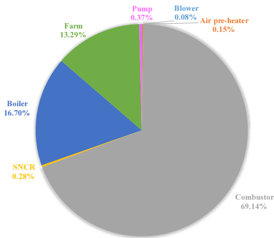
Fig. 5. Exergy destruction ratio for individual components
