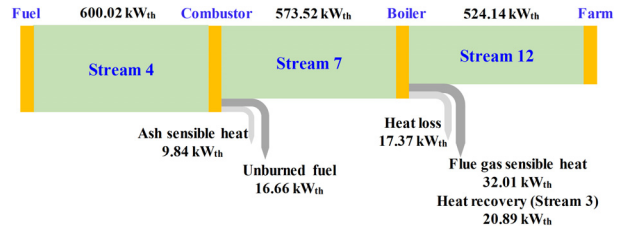
Fig. 2. Energy flow diagram of the livestock manure solid fuel combustion boiler system
