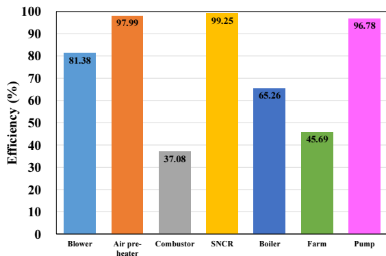
Fig. 4. Exergy efficiencies for individual components
