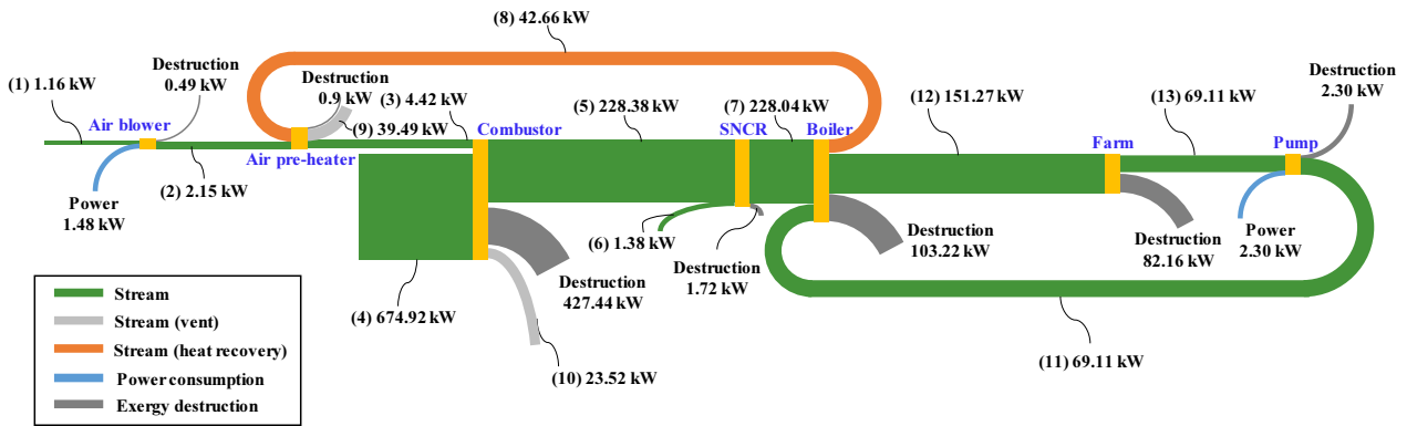
Fig. 3. Exergy flow diagram of the livestock manure solid fuel combustion boiler system
